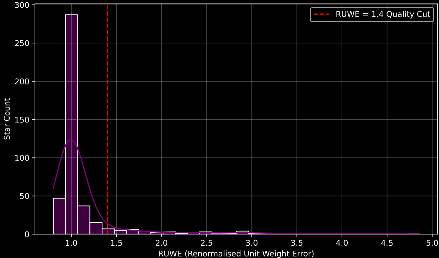
GAPOGEE DR17 Field [GD1-3] RUWE Distribution (n= 434)
