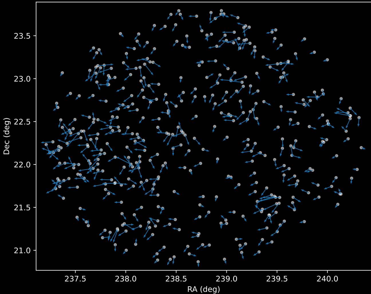
APOGEE DR17 Cluster 0 Proper Motion Vectors (n=418)
