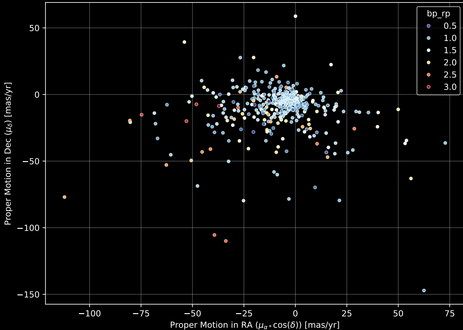
APOGEE DR17 Field: [GD1-3] Proper Motion Diagram (n= 448)
