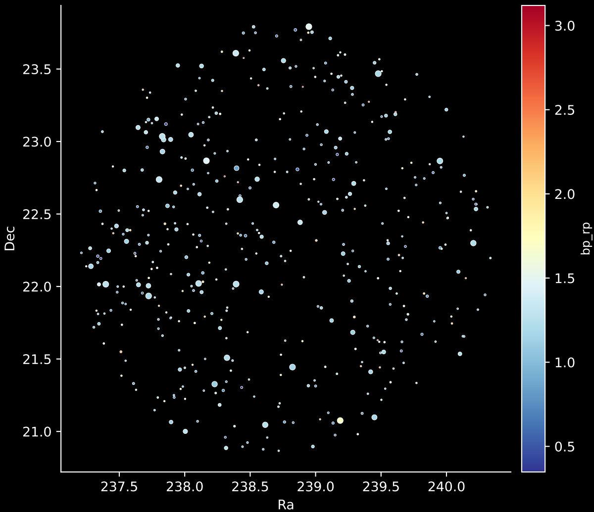
APOGEE DR17 Field: [GD1-3] Stars: 448
