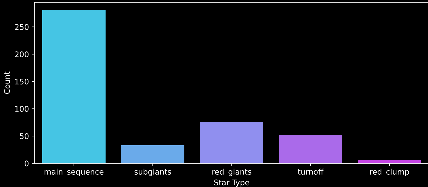
APOGEE DR17 Field: [GD1-3] Count plot of Star Type
