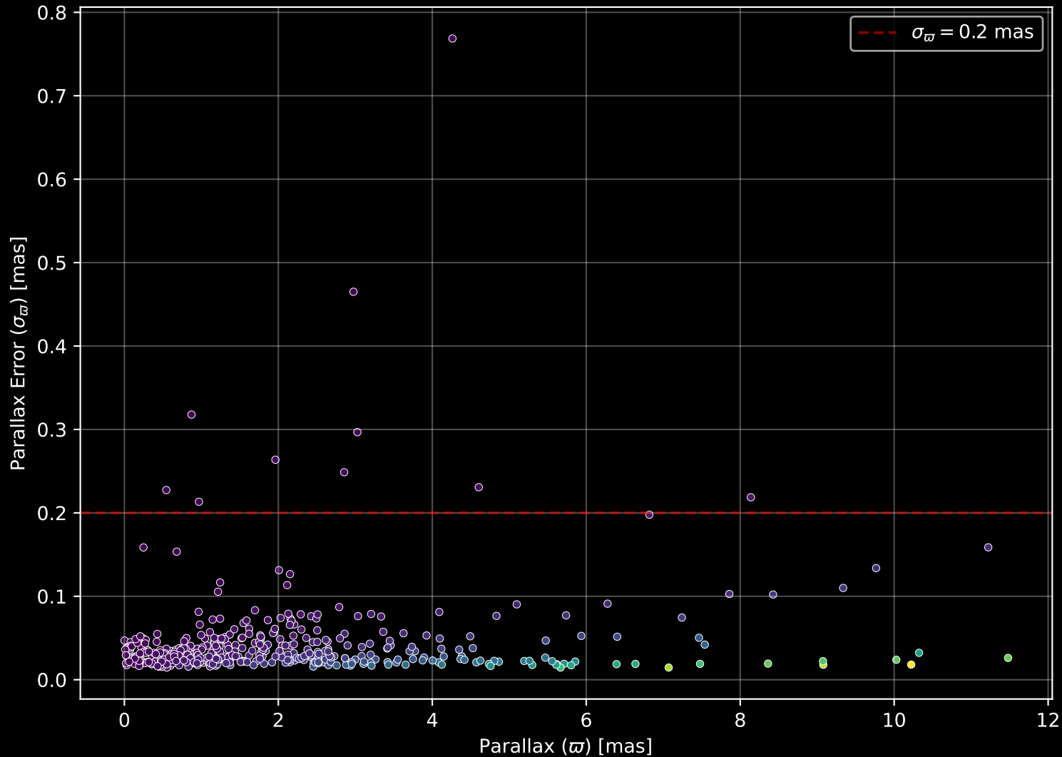
APOGEE DR17 Field: [GD1-3] Parallax Quality (n= 448)
