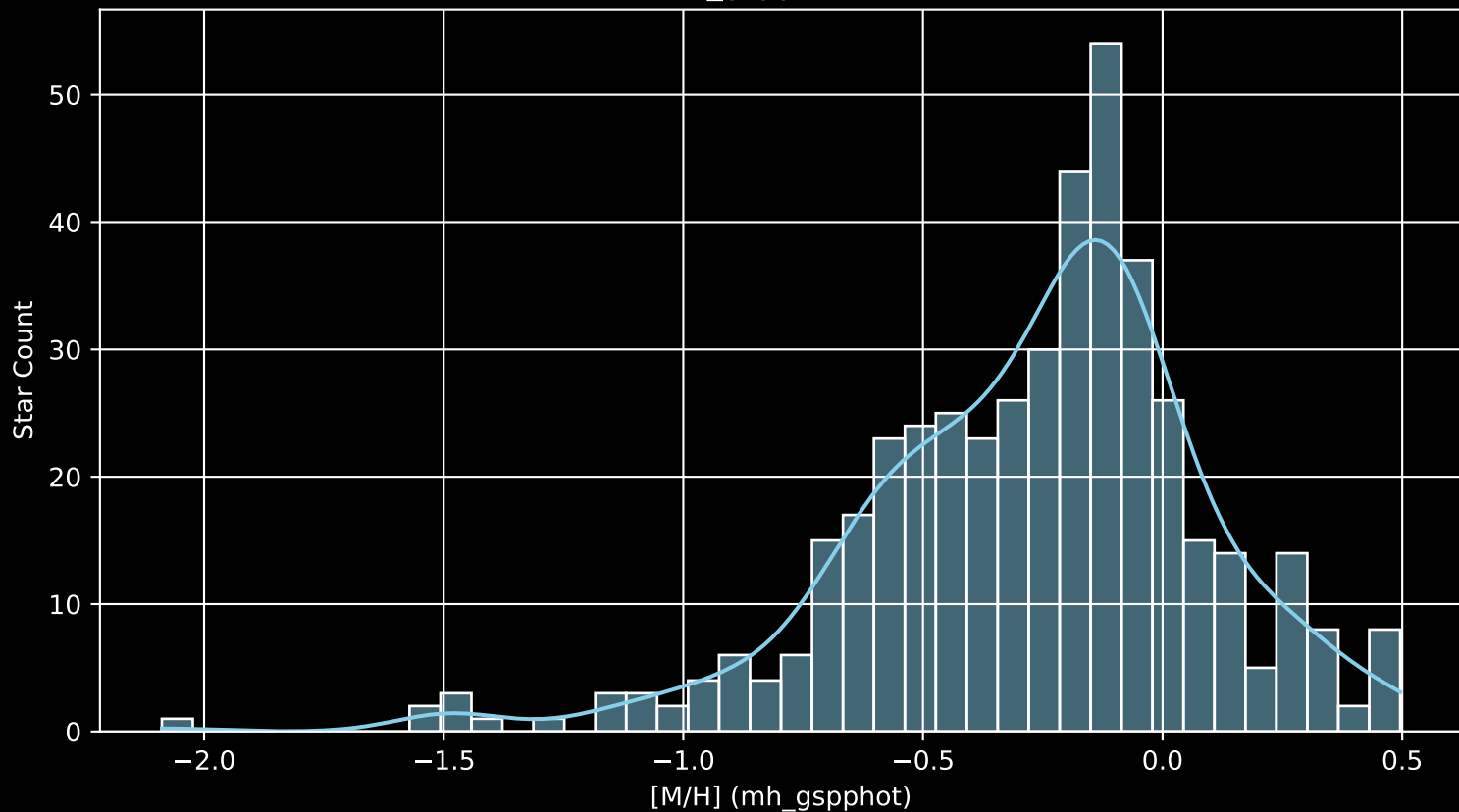
APOGEE DR17 Field: [GD1-3 [M/H] (mh_gspphot) (n= 446)
